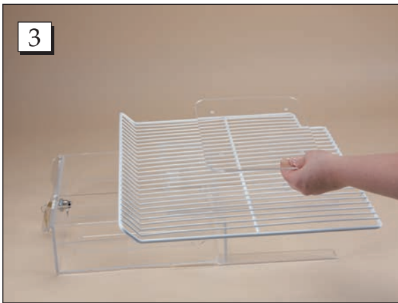
Step 3. Place the retention plate on top of refrigerator shelf.
